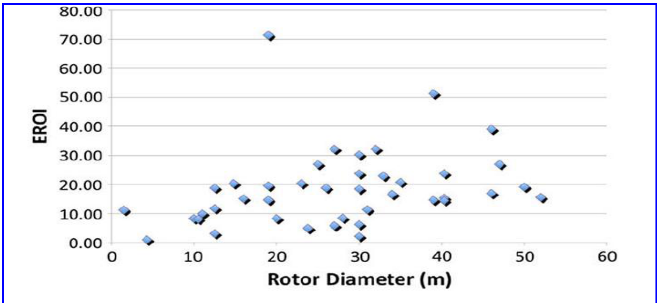
Figure 5.8 Rotor size to EROEI (Kubiszewski et. al. ibid. fig.4 p224)
